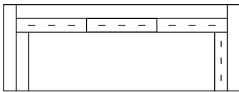
85832 L ARM CORNER SOFA TOTAL W89" D35" H34" SEAT W76" D21" H19" ARMS --- --- H28"
