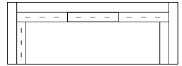
85831 R ARM CORNER SOFA TOTAL W89" D35" H34" SEAT W76" D21" H19" ARMS --- --- H28"
